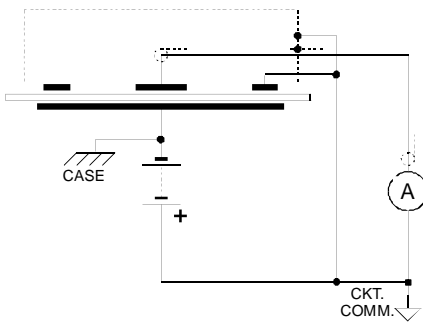
Figure 3: Setup for Guarded Measurement of Volume Resistivity
